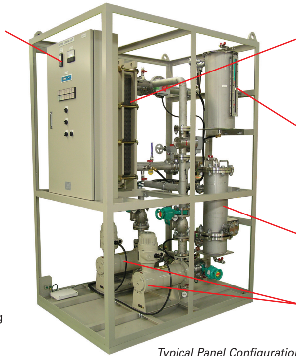
Typical Panel Configuration
