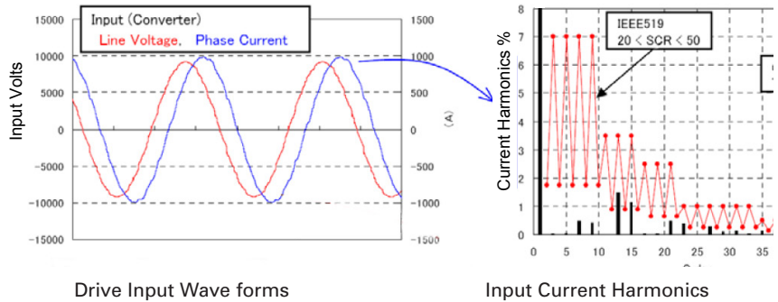
Drive Input Wave forms
